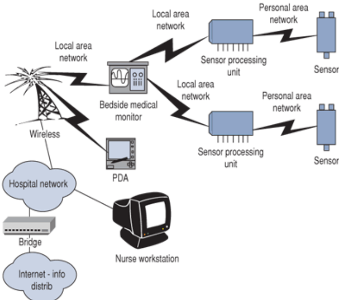
Figure 1 In this medical monitoring system example, the sensor measures the desired parameter and transmits this data to the sensor processing unit. The unit processes the output from the sensor and produces a data stream compatible with the bedside monitoring station. The combined data from this unit can also be transmitted over a network to a nurses station as well as to a central server for data storage and information distribution.
